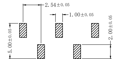
Recommended PCB Layout SM2 TYPE
