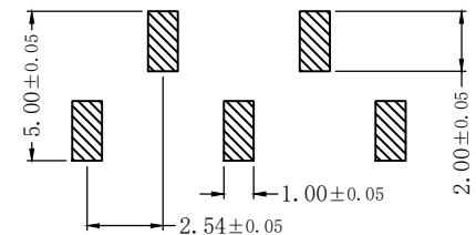
Recommended PCB Layout SM1 TYPE
